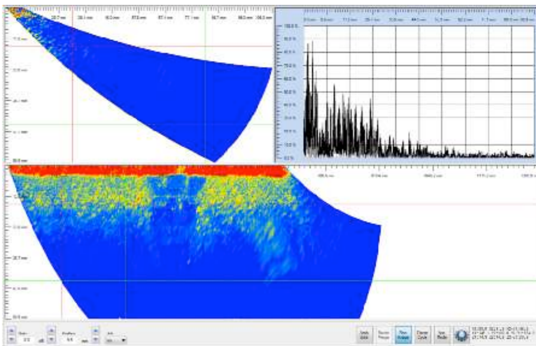
Perpendicular scan to the weld
