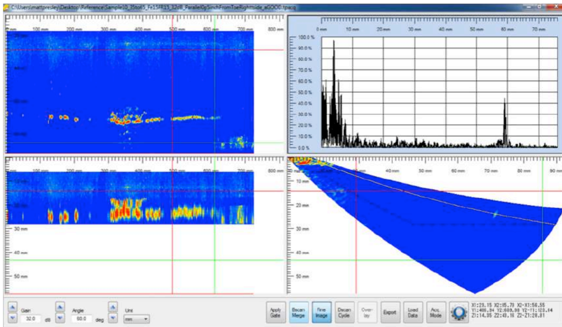
Parallel scan to the weld
